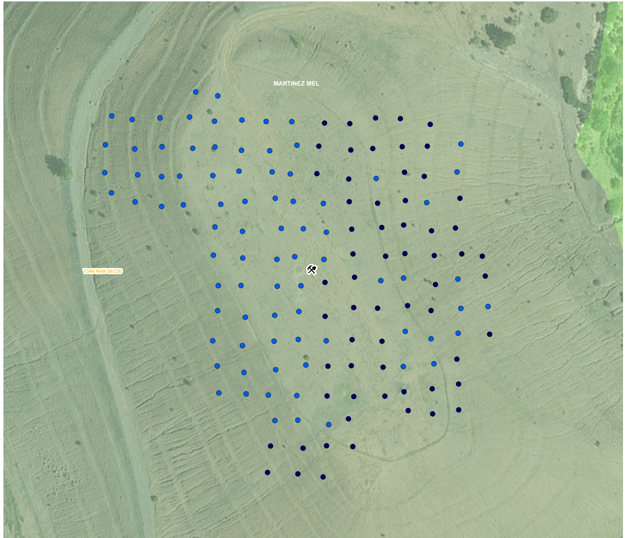
FIGURE 38 SURFACE TEMPERATURE MEASUREMENTS CHIMNEY ROCK MINE 2013 OUTCROP ZONE REPORT ARCHULETA COUNTY, COLORADO PETROX RESOURCES AND ELM RIDGE RESOURCES
