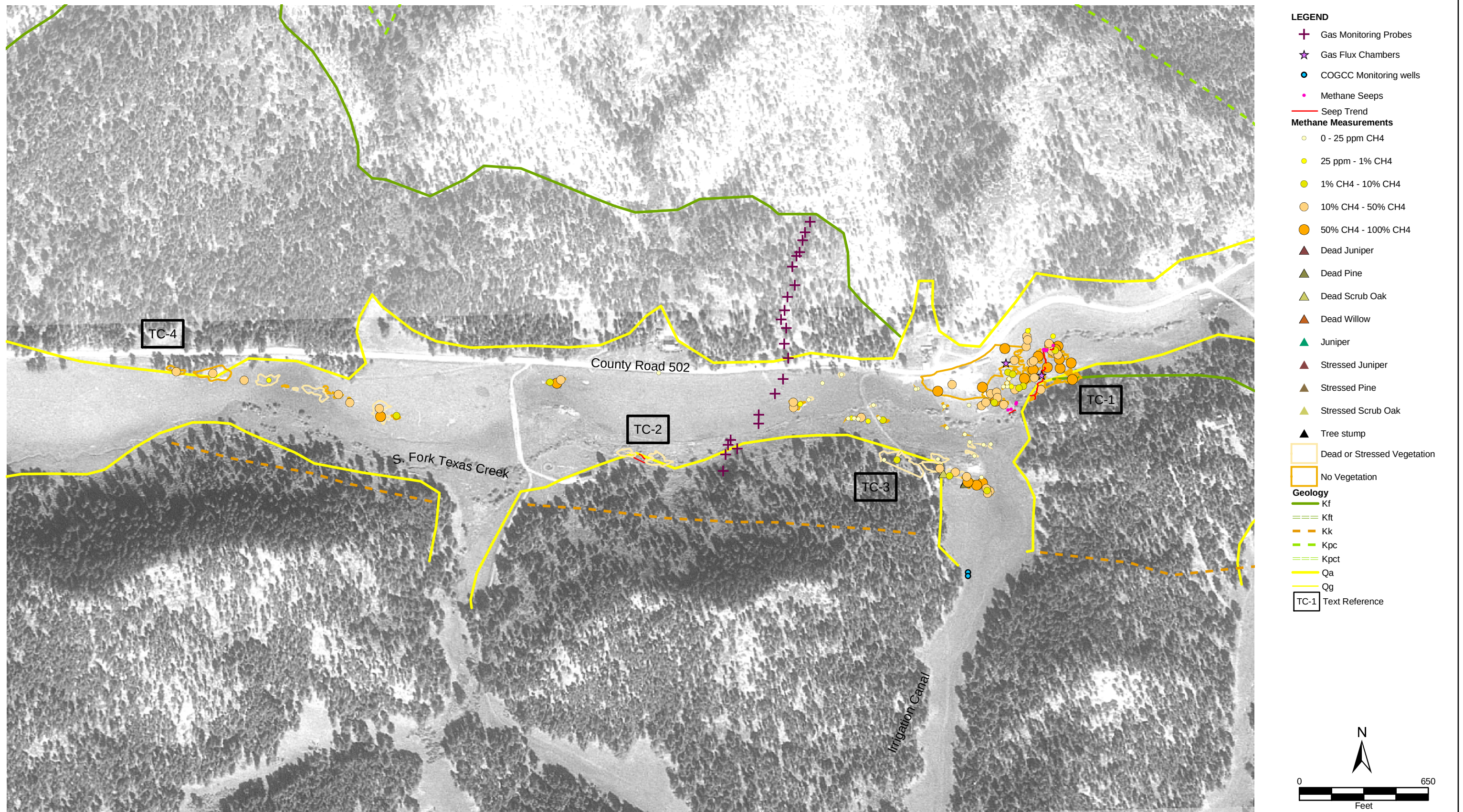
FIGURE 16 2004 DETAILED SEEP MAPPING TEXAS CREEK WEST THE GROUP
