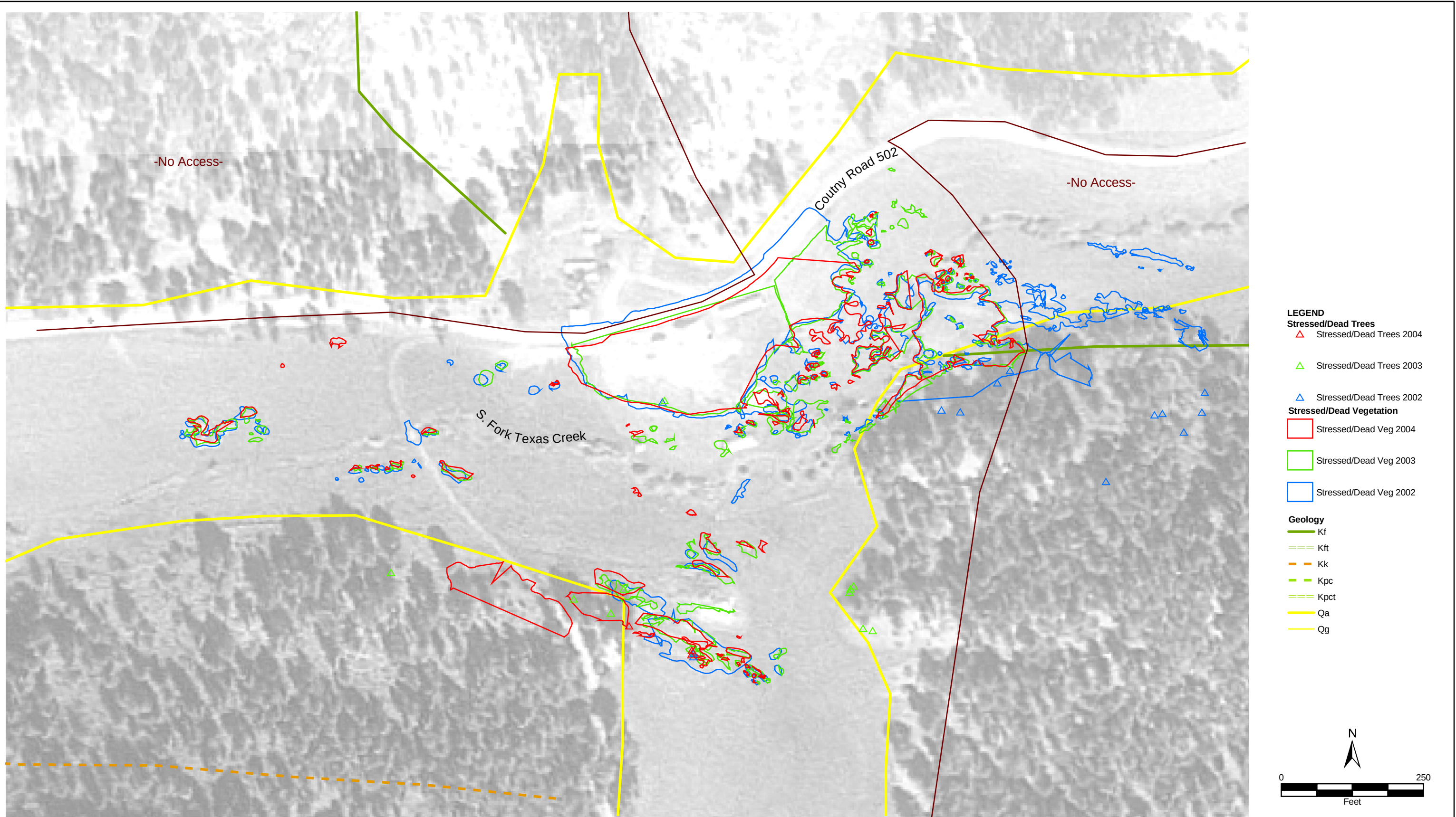
FIGURE 22 HISTORICAL DATA COMPARISON STRESSED/DEAD VEGETATION TEXAS CREEK (detail) THE GROUP
