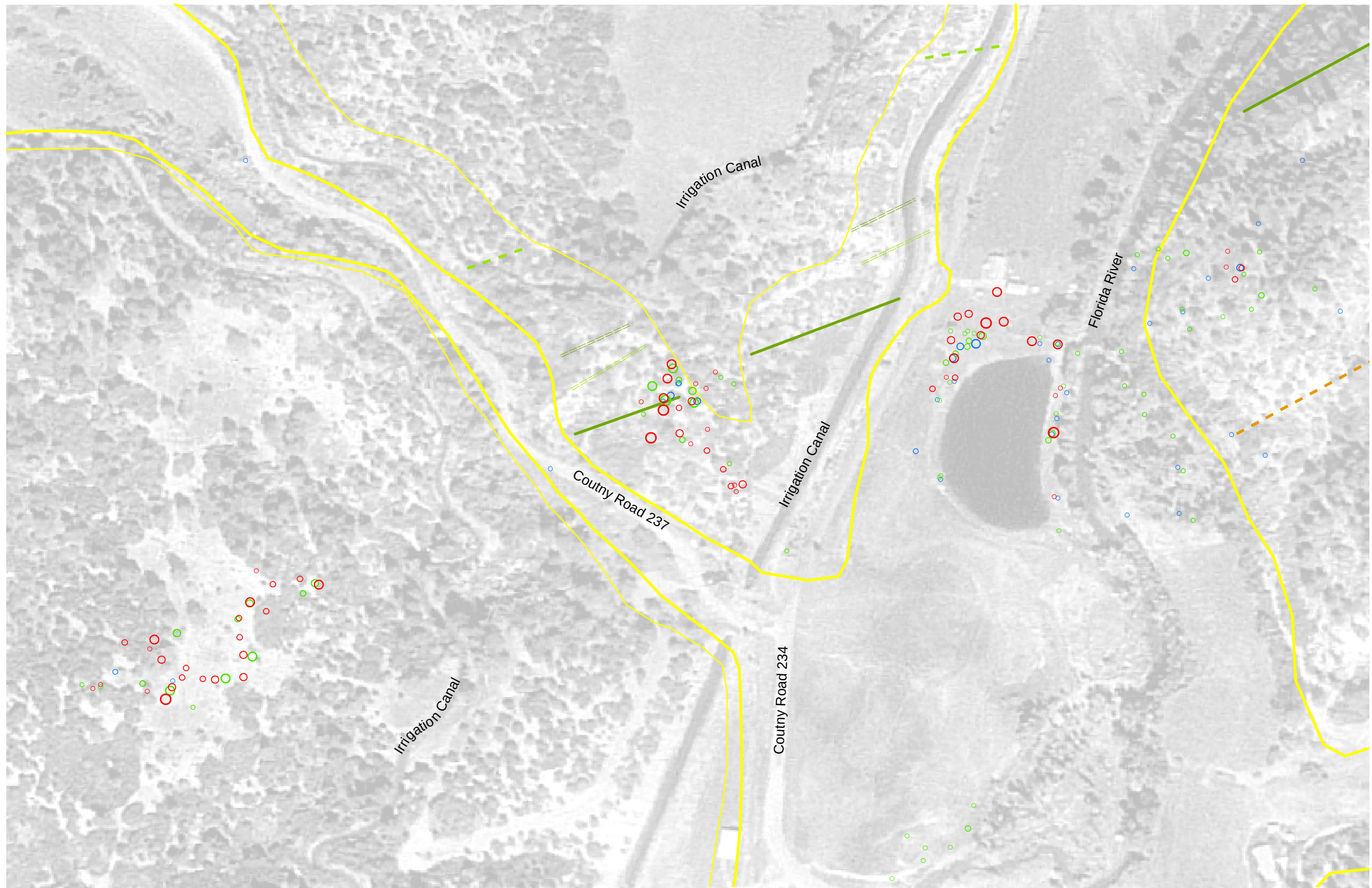
FIGURE 13 HISTORICAL DATA COMPARISON SUBSURFACE METHANE MEASUREMENTS FLORIDA RIVER THE GROUP
