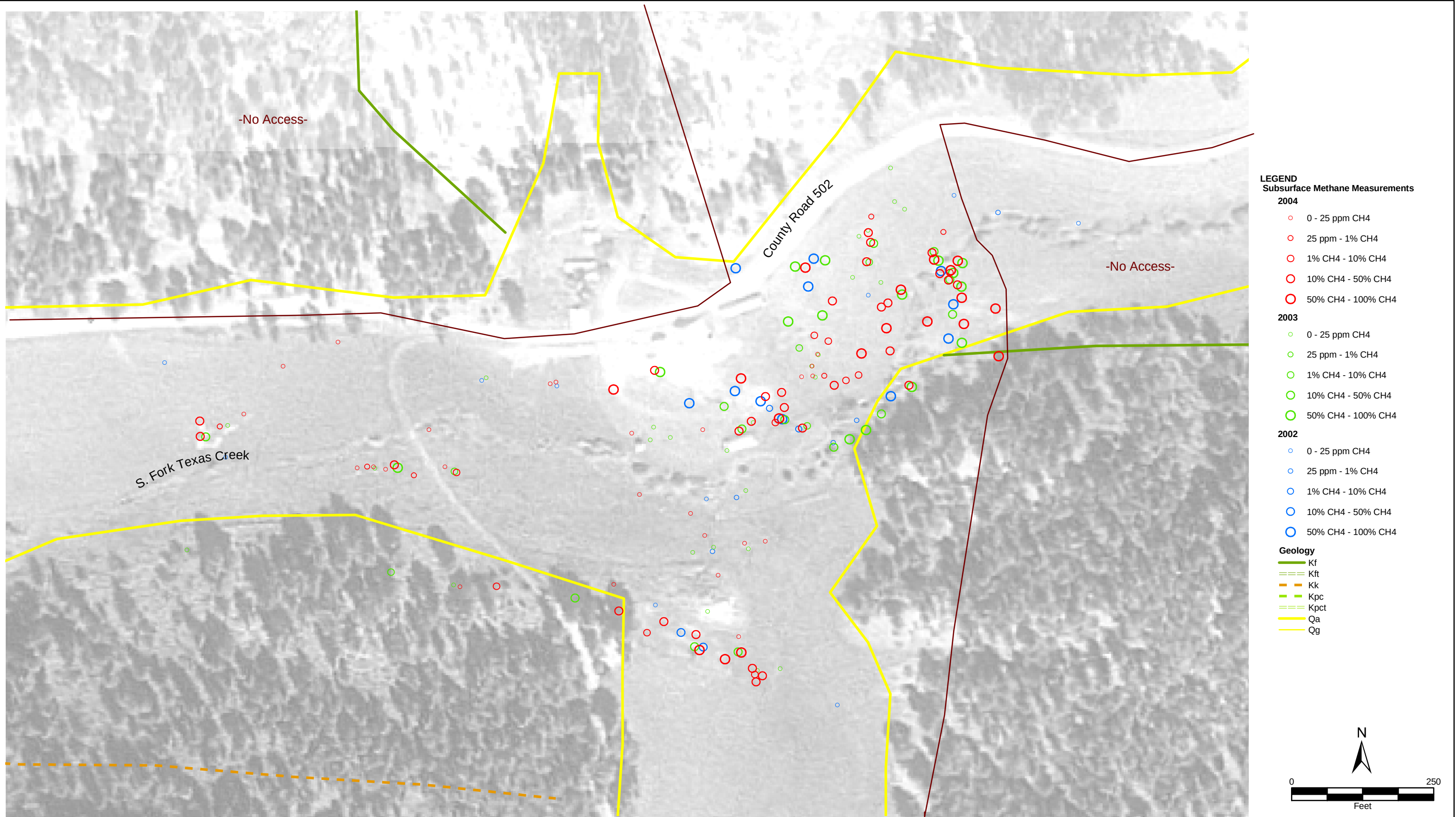
FIGURE 20 HISTORICAL DATA COMPARISON SUBSURFACE METHANE MEASUREMENTS TEXAS CREEK (detail) THE GROUP
