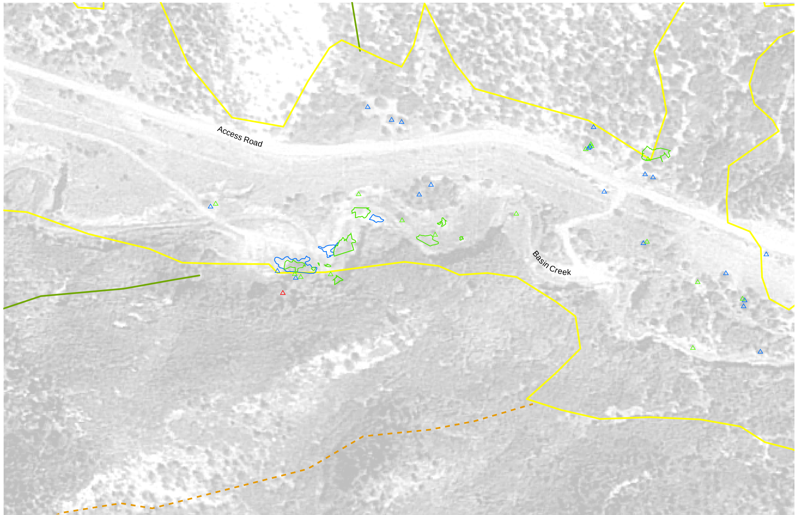
FIGURE 4 HISTORICAL DATA COMPARISON STRESSED/DEAD VEGETATION BASIN CREEK THE GROUP
