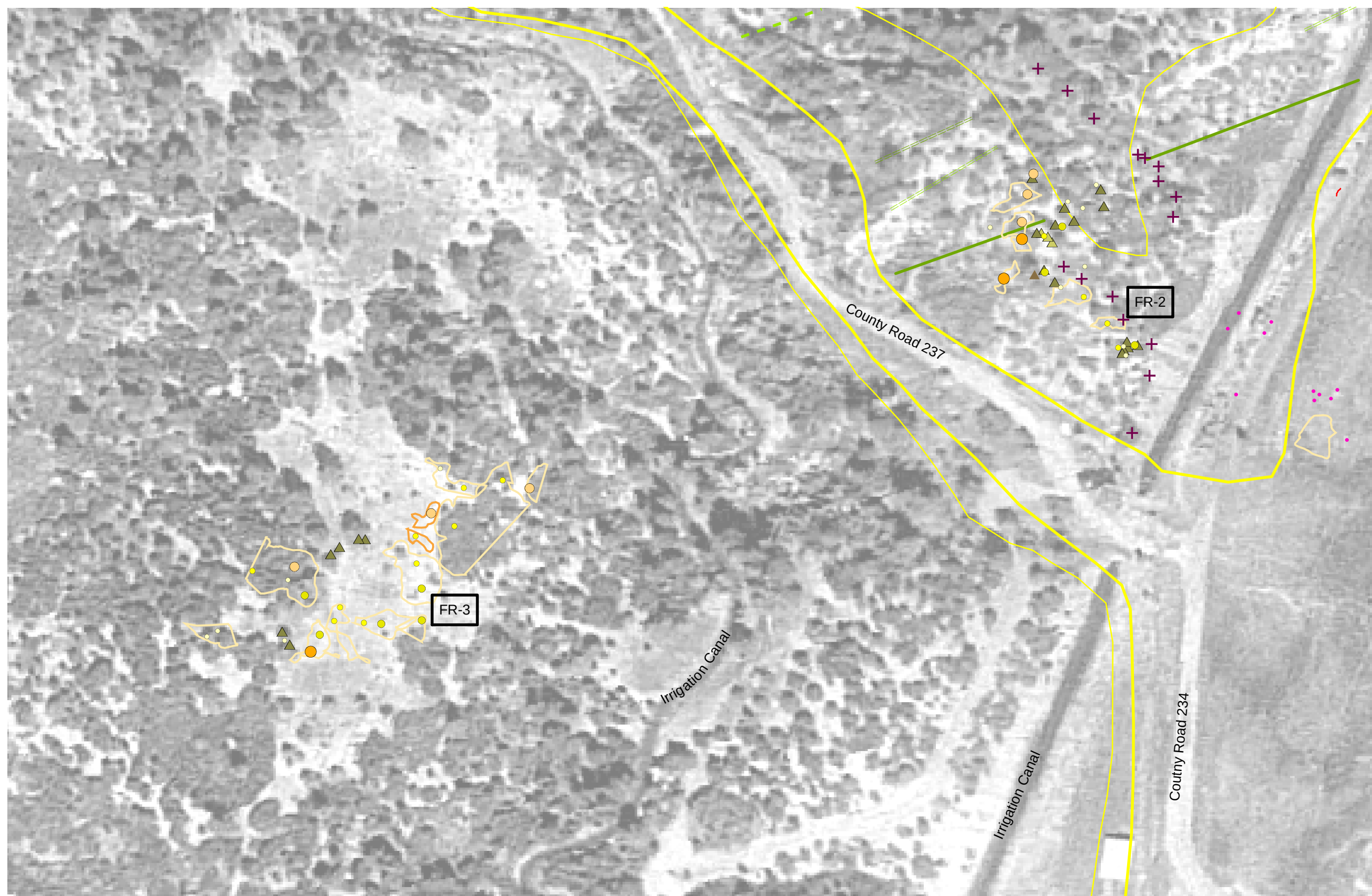
FIGURE 11 2004 DETAILED SEEP MAPPING FLORIDA RIVER WEST THE GROUP
